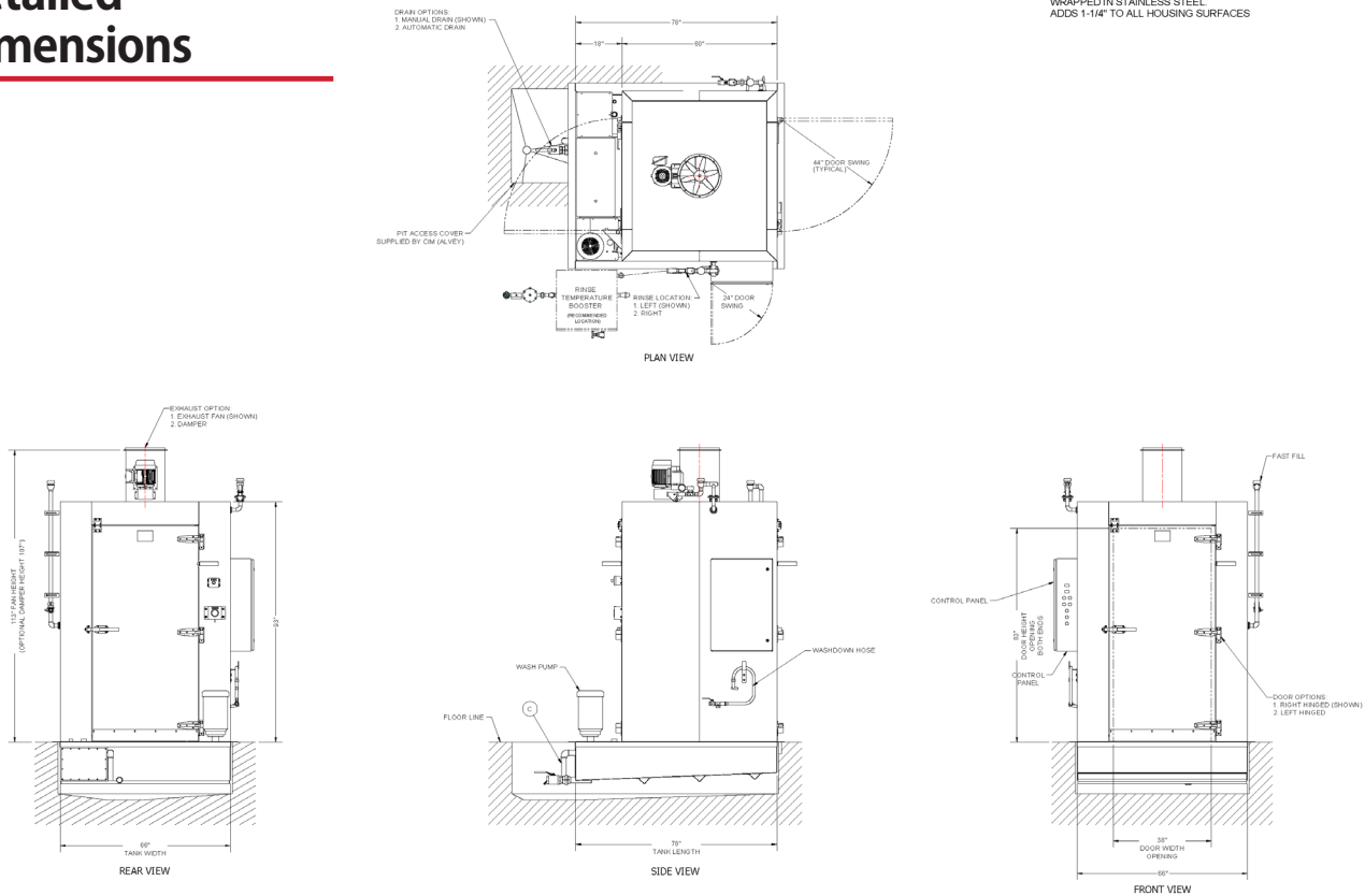
KS-70 PIT MOUNT, PASS THROUGH, ELECTRIC HEAT
