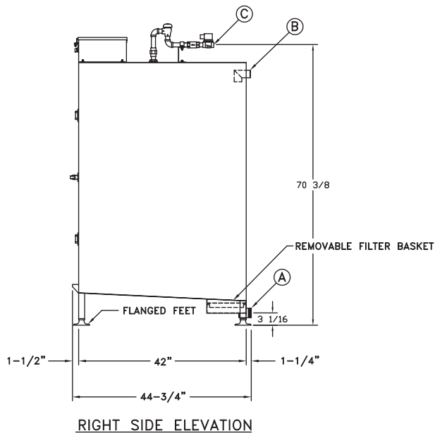
RIGHT SIDE ELEVATION
